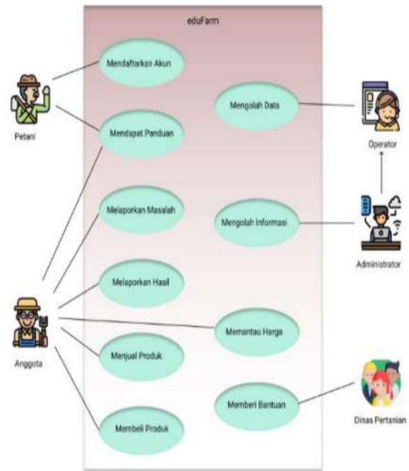
Gambar 1. Use Case Diagram eduFarm
