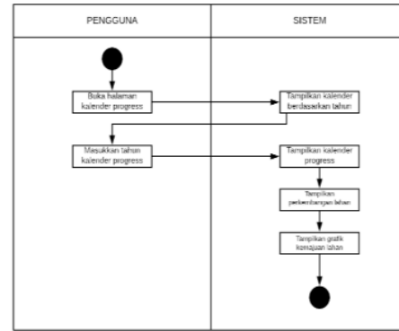
Gambar 4. Activity Diagram Detail Lahan Kosong
