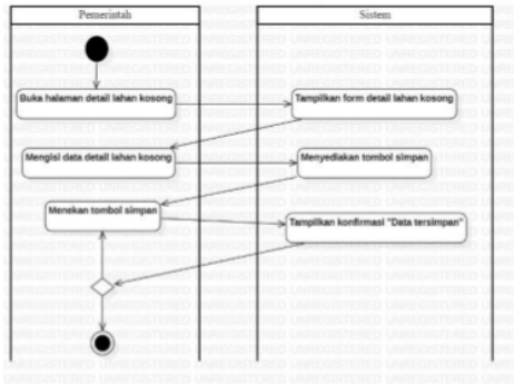
Gambar 2. Activity Diagram Detail Lahan Kosong
