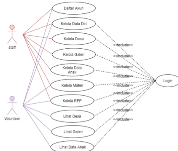
Gambar 1.1 Tampilan Use case diagram Pendar
