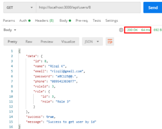
Gambar 7. Response API /api/users/:id
