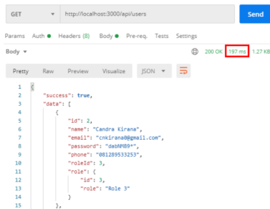
Gambar 8. Response API /api/users
