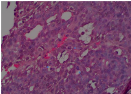
Gambar 1. Sel Mitosis
