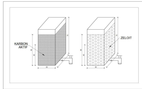
Gambar 1. Reaktor Penelitian
