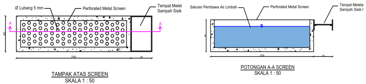
Gambar 4. Desain Perforated Metal Screen
