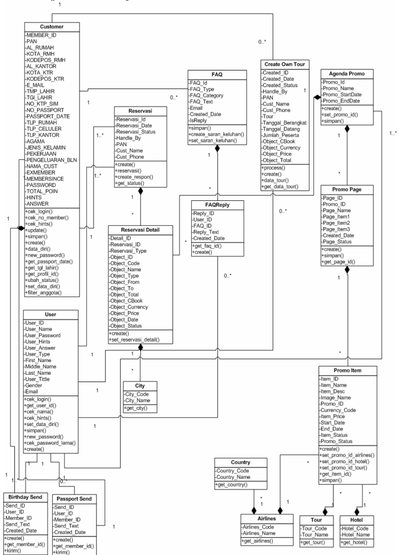
Gambar 4. Class Diagram E-CRM PT. Fajar Buana Internasional
