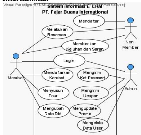
Gambar 3. Use Case Diagram E-CRM PT. Fajar Buana Internasional
