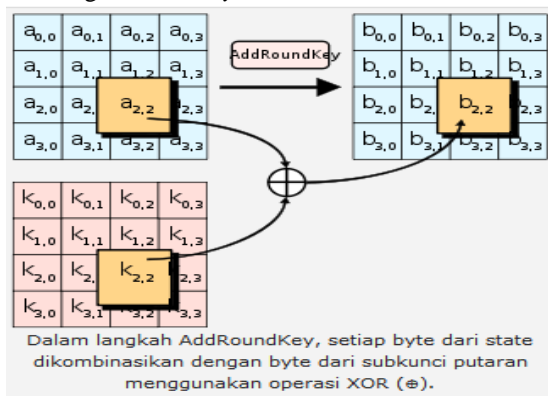
Gambar 6. AddRoundKey
