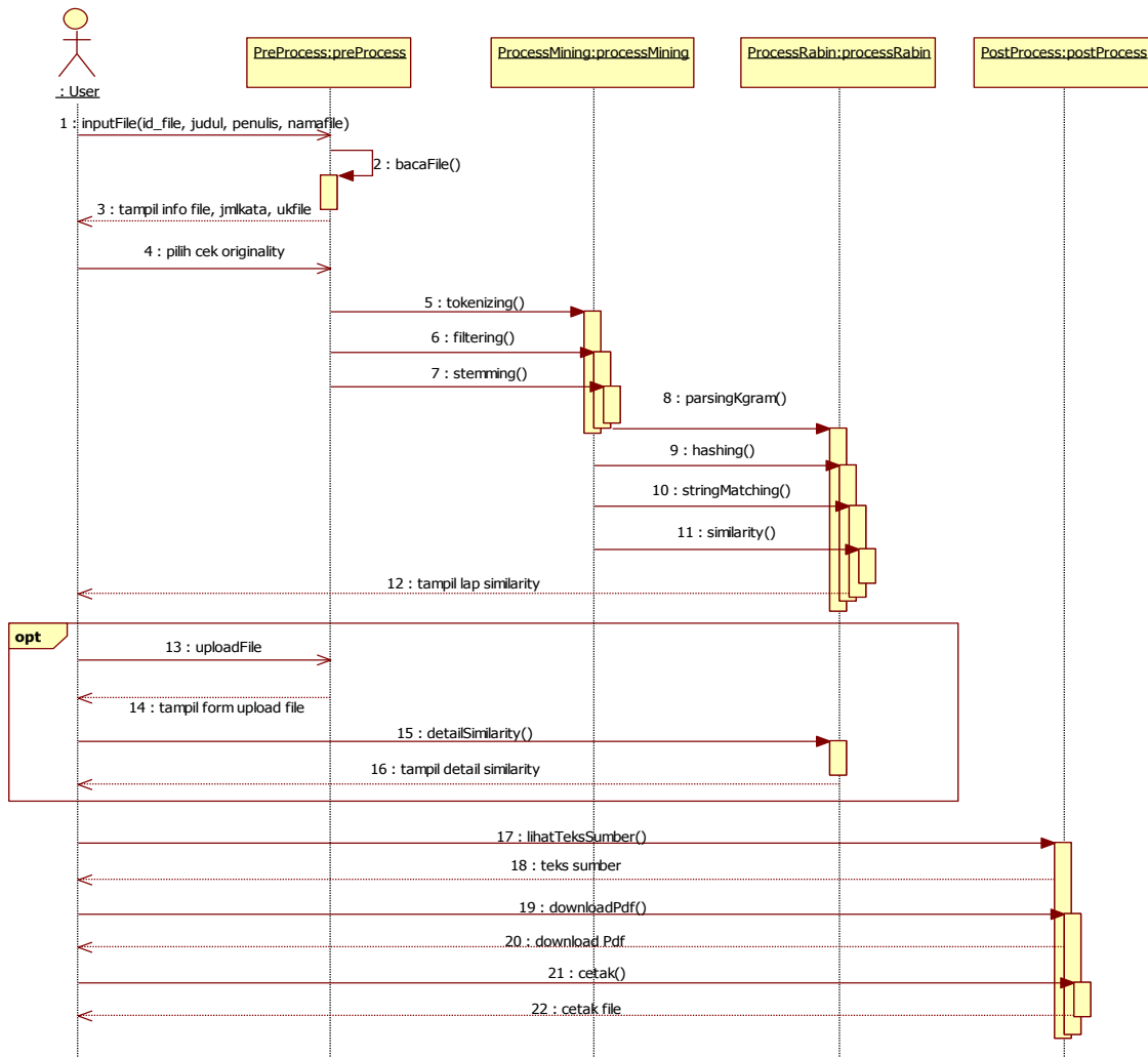
Gambar 5. Sequence diagram
