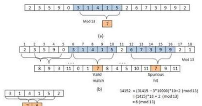
Gambar 1. Algoritma Rabin Karp
