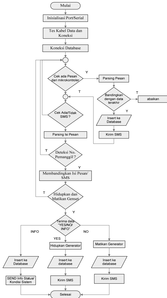
Gambar 6. Flowchart Algoritma Penampil
