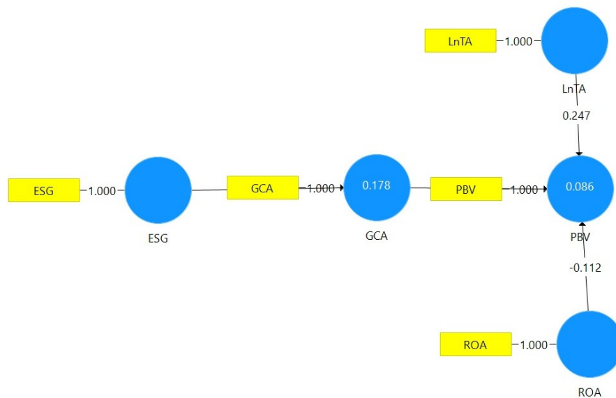
Figure 2. PLS Model Result
