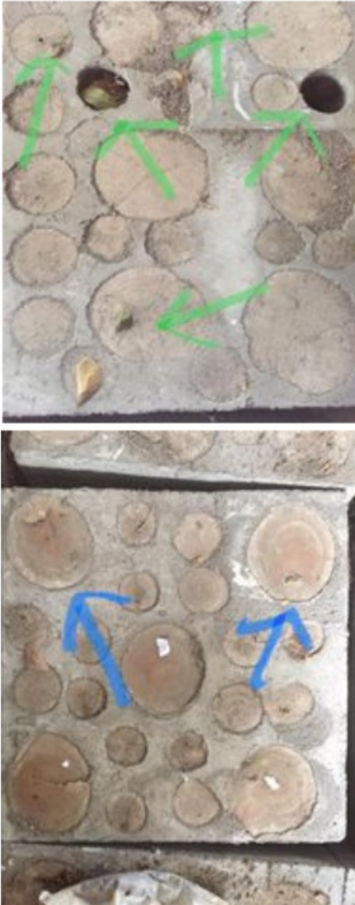
Figure 4. Condition of the top side of the floor block after 5 months
