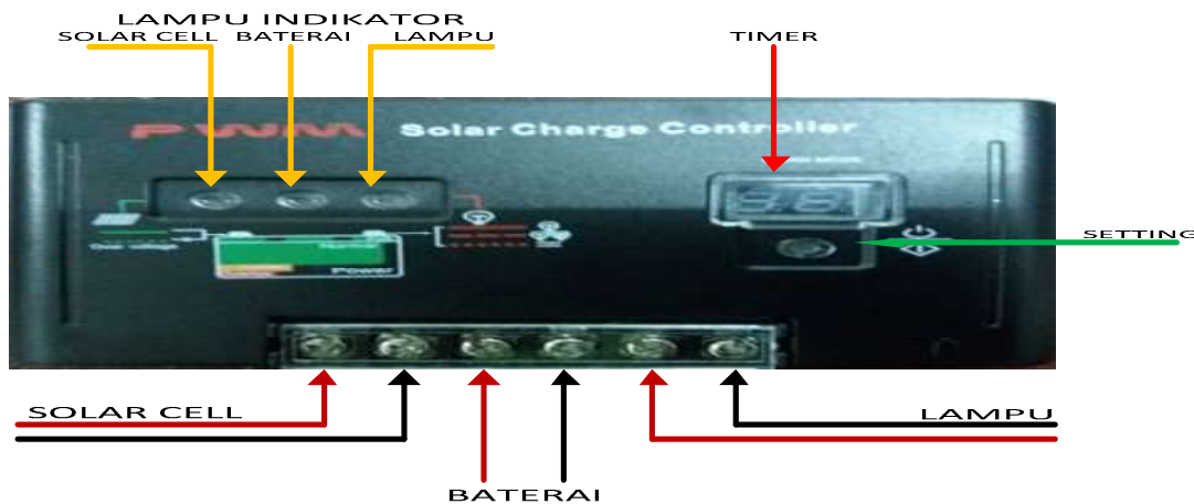
Gambar 8. Solar Charger Controller.
