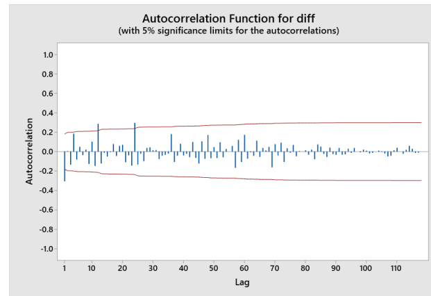
Gambar 6. Plot ACF Data Differencing
