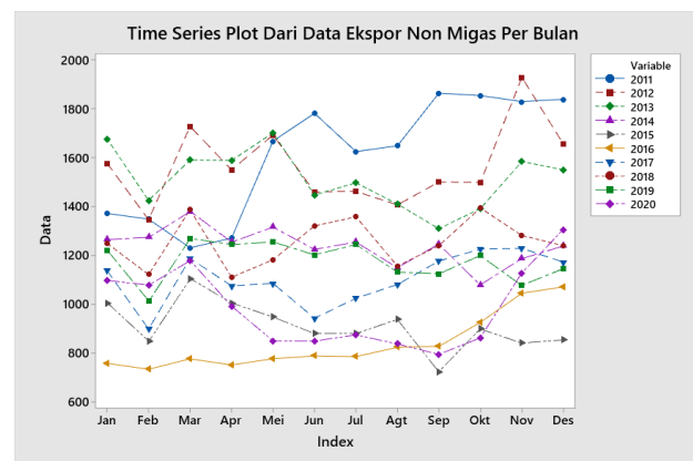
Gambar 2. Time Series Plot Per Bulan
