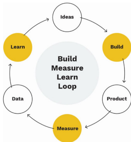
Gambar 1. Siklus Build-Measure-Learn
